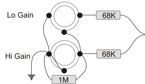
Layout Diagram
